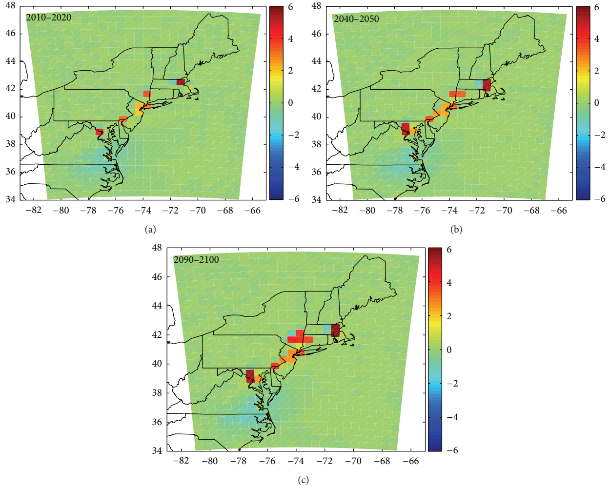
FIGURE 3: Effects of future urban expansion on average annual temperature in the Northeast megalopolis, USA (unit: °C).
